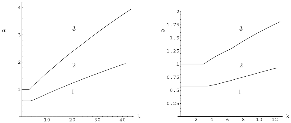
FIG. 1. Stationarity regions for model (1.2) with \eta_t \sim \mathcal{N}(0, 1) . 1. Existence of E\varepsilon_t^4 ; 2. Existence of E\varepsilon_t^2 with E\varepsilon_t^4 = \infty ; 3. Strict stationarity with E\varepsilon_t^2 = \infty . The right panel is a zoom of the left panel.
