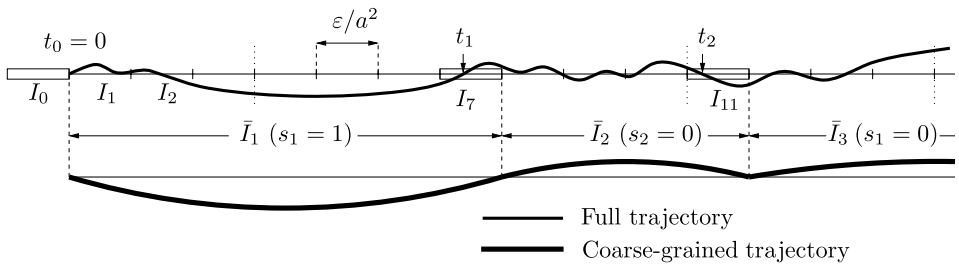
FIG. 3. A full trajectory, on top, and the corresponding coarse-grained trajectory, below. The visited blocks are surrounded by a box and the first renewal point inside such blocks is marked by a vertical arrow: a coarse-grained excursion is everything that lies between visited blocks. One stipulates that there is a visited block to the left of the origin, containing the origin. The visited block on the right belongs to the coarse-grained excursion, while the one on the left does not. The sign of the excursion is just the sign of the full trajectory just before the vertical arrow (except possibly for the last excursion). In this example \delta/\epsilon = 4 , so the first three blocks to the right of a visited block (i.e., up to the vertical dotted lines) cannot be visited blocks.
