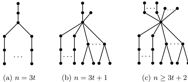
Figure 1.1: Trees in \mathcal{T}_1(n, \psi) .
