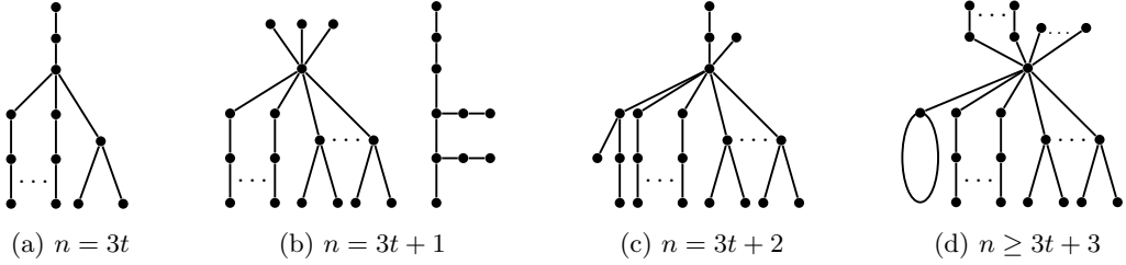
Figure 1.2: Trees in \mathcal{T}_2(n, \psi) , and the ellipse in the last graph stands for P_{2l} with l \in \{2, 3\} .
