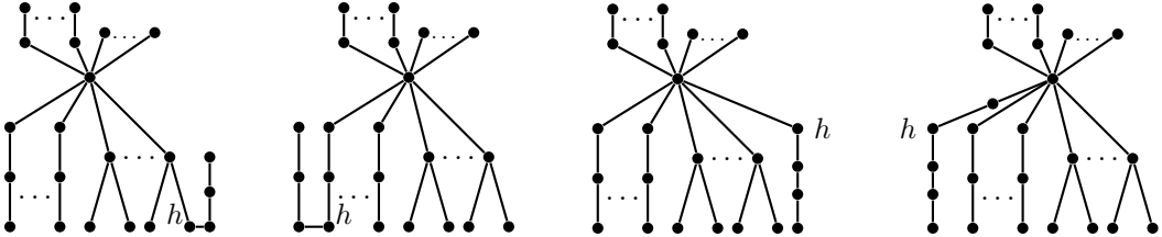
Figure 3.3: All possible structures of T_0 if x = 1 and T_2 \in \mathcal{T}_1(n_2, \psi_2) with n_2 \geq 3t_2 + 3 .
