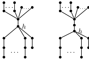
Figure 3.2: All possible structures of T_0 for x = t_0 - 2 .
