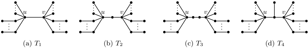
Figure 3.1: All possible structures of T if n - \psi = 2 .
