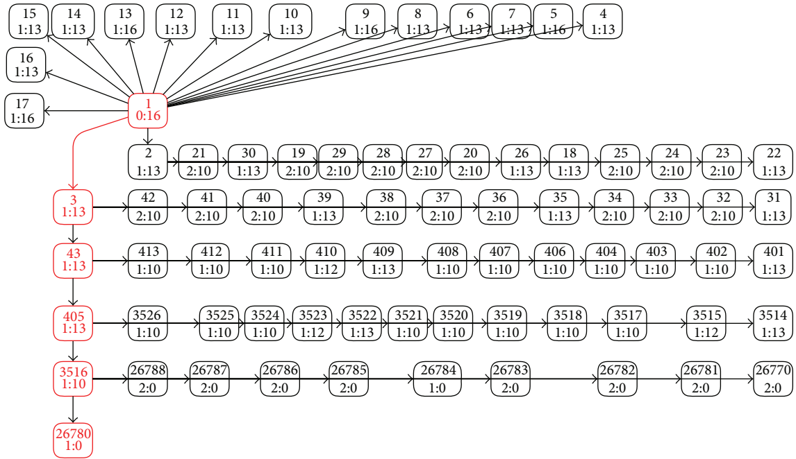
FIGURE 8: State space analysis, O^{26780} .
