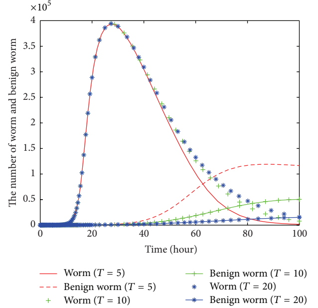
FIGURE 19: Comparison of different T .
