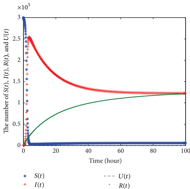
FIGURE 21: Worm infection status.
