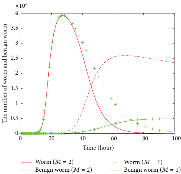
FIGURE 18: Comparison of different M .
