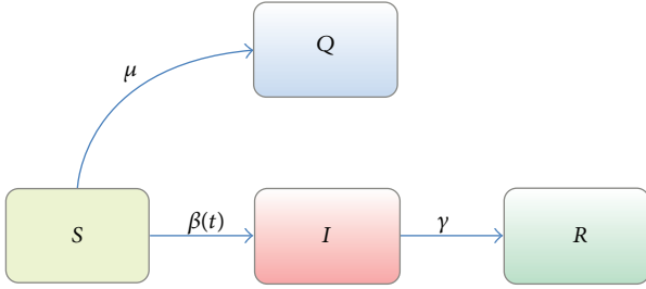
FIGURE 3: State transition of TF mode.
