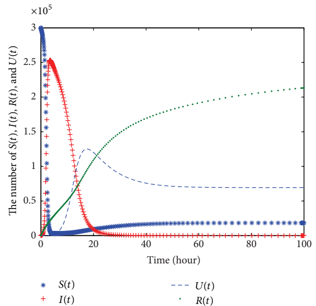
FIGURE 23: Interaction infection state.
