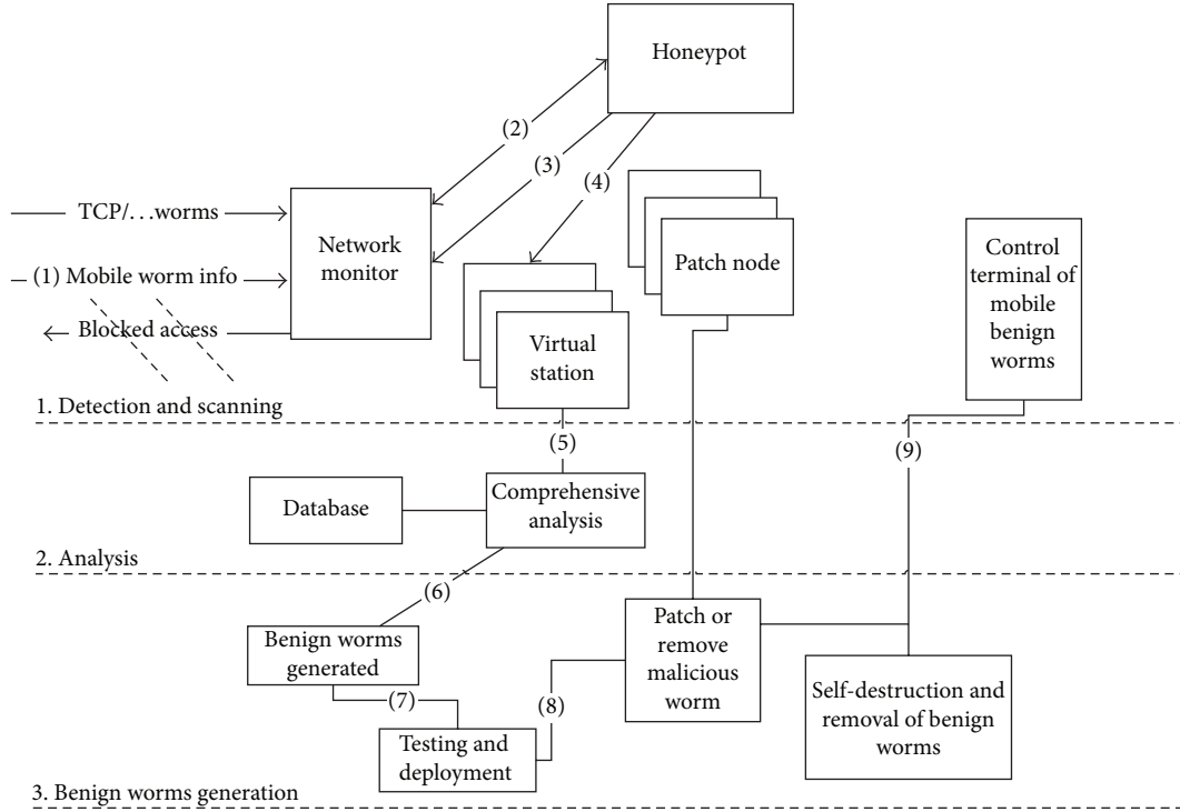
FIGURE 5: Benign worm mechanism based on honeypot.
