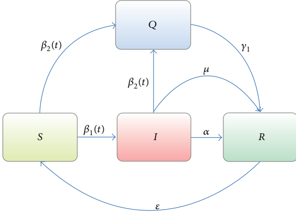
FIGURE 9: State transition of Situation 3.
