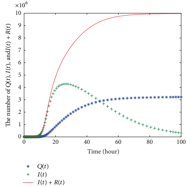
FIGURE 4: The simulation of TF mode.
