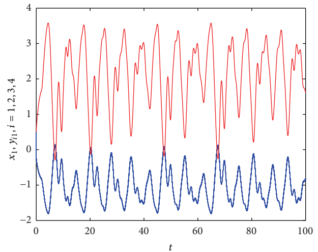
FIGURE 3: The trajectories of state variables with \lambda = -0.5 .
