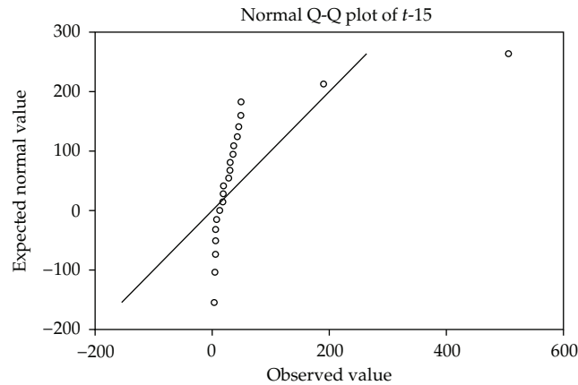
Figure 3: Q-Q of potential differences detected at time t = 15 s during the same seizure. Note that the data no longer displays normal tendencies.
