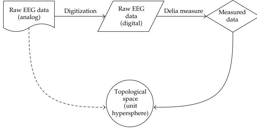
Figure 4: Pathway to mapping EEG signals to a manifold.
