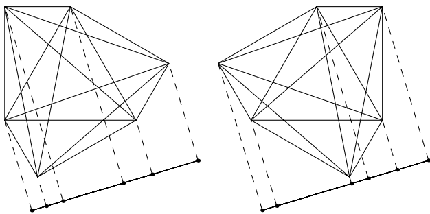
FIGURE 1. An autometric set of points and a corresponding pair of homometric Golomb rulers (see Section 7).
