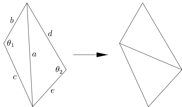
FIGURE 7. The two adjacent triangles on the left violate the equiangularization criterion, since we have \theta_1 + \theta_2 > \pi . Equiangularization flips the quadrilateral diagonal, making the triangles more nearly equiangular.
