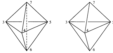
Fig. 2. Two different triangulations T_A (left) and T_B (right) for the models X_7(7, 3, 2, 1, 1) In the left, we see three 3-simplices whereas in the right we see two 3-simplices This results in different regular fans \Sigma(\Delta^*)^A_{\text{reg}} and \Sigma(\Delta^*)^B_{\text{reg}} for the different desingularizations of the ambient space However the Calabi–Yau hypersurfaces in them have the same topology
