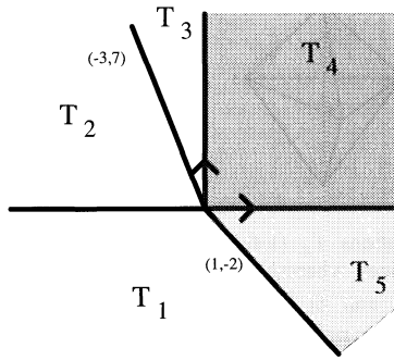
Fig. 3. The secondary fan for the polyhedron \Delta^*(7,3,2,1,1) . The Kähler cones of the smooth ambient spaces \mathbf{P}_{\Sigma(\Delta^*)^A_{\text{reg}}} and \mathbf{P}_{\Sigma(\Delta^*)^B_{\text{reg}}} have different restrictions to the secondary fan. The restricted Kähler cone for the former space is given by the union of the cones parametrized by T_4 and T_5 , while for the latter it is given by the cone parametrized T_4 .
