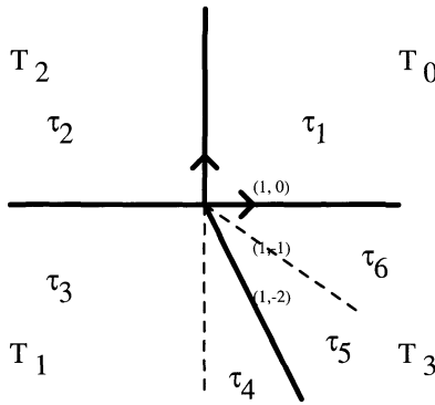
Fig. 1. The secondary fan and the Gröbner fan for \mathbf{P}(2,2,2,1,1) The secondary fan consists of the polyhedral cones parametrized by the regular triangulations T_0, \dots, T_3 in the text. The Gröbner fan provides a refinement consisting of \tau_1, \dots, \tau_6 represented by the typical weights in Table 1
