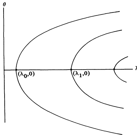
FIGURE 2.5. Bifurcation diagram for (2.1), (2.4).
