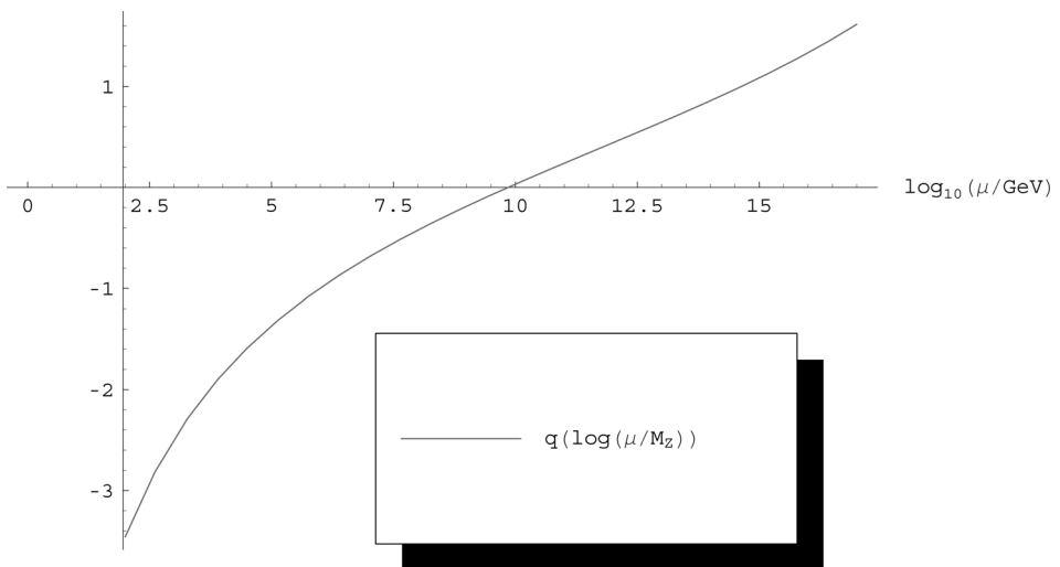
Figure 7: The running of the tadpole term.
