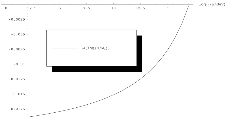
Figure 5: The running of the ratio of the coefficients of the R^2 term and the Weyl term in (5.31).
