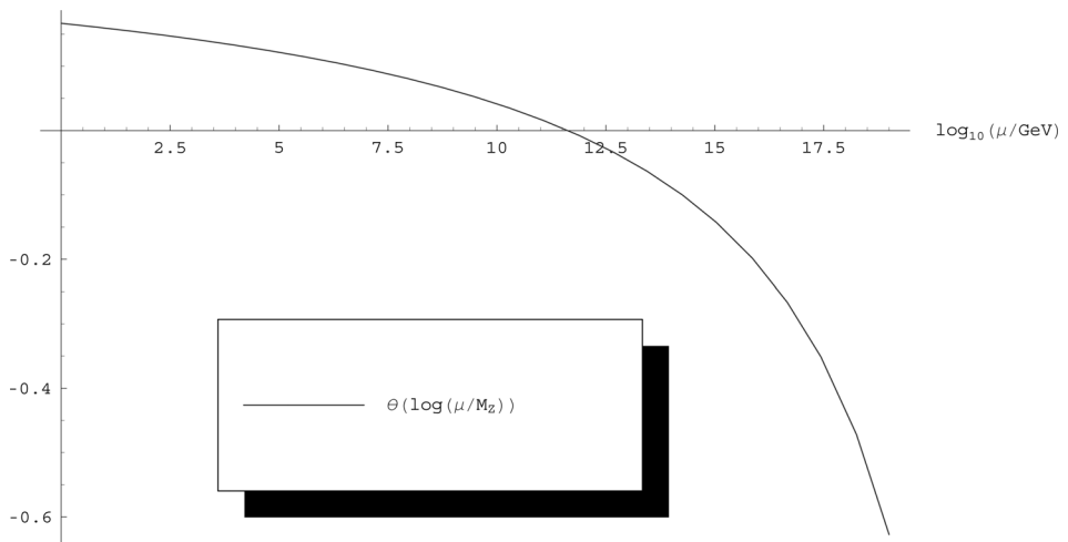
Figure 6: The running of the ratio of the coefficients of the topological term and the Weyl term in (5.31).
