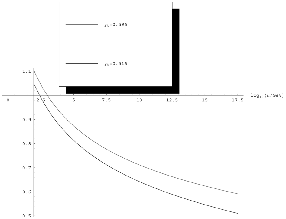
Figure 3: The running of the top quark Yukawa coupling.
