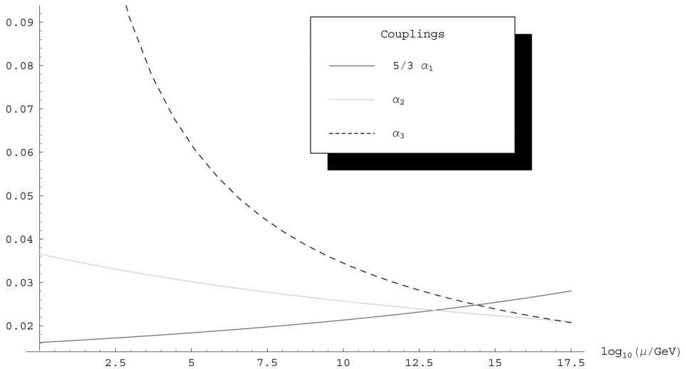
Figure 1: The running of the three couplings.
