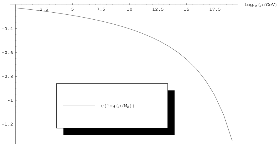
Figure 4: The running of the Weyl curvature term in (5.31).
