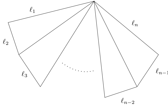
FIG. 5. The triangulation associated to \Gamma_n
