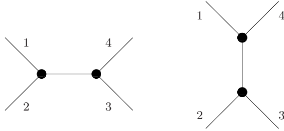
FIG. 7. The graphs \Gamma and \Gamma'
