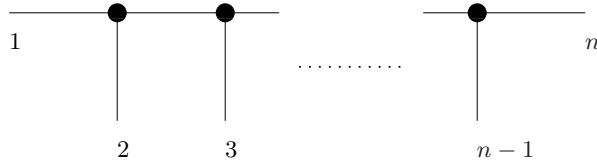
FIG. 4. The graph \Gamma_n
