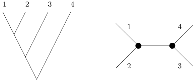
FIG. 3. A tree and its associated admissible graph
