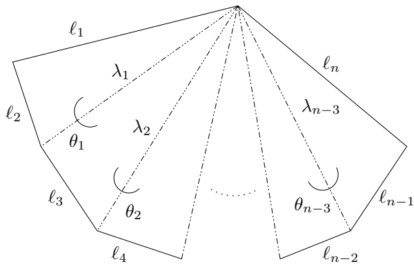
FIG. 1. Action-angle coordinates (\lambda_i, \theta_i)_{i=1, \dots, n-3} .
