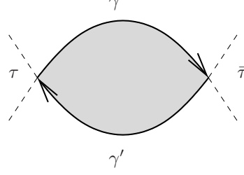
FIG. 9. The domain D(E, E')
