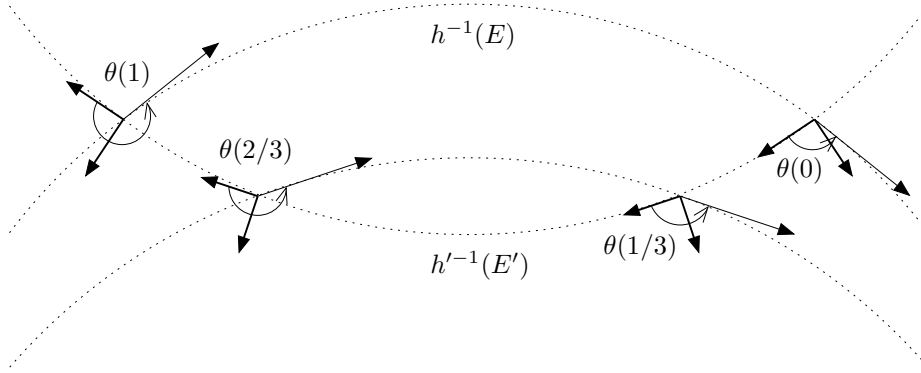
FIG. 10. the angle \theta
