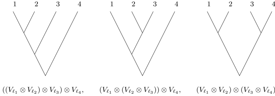
FIG. 2. The graphs associated to various parenthesisings
