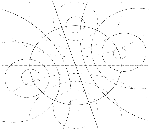
FIG. 8. The two fibrations and the circle C
