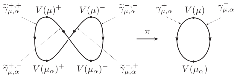
Fig. 1. Projections of gradient trajectories.
