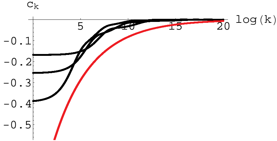
FIGURE 7. Plot of c_k if \alpha = \frac{\beta}{4} + \frac{1}{2} for \beta = 6, 8, 10 [black curves from the bottom to the top] and the reference function -k^{-\frac{1}{4}} [red curve] (data obtained with n = 10^6 in (4)).
