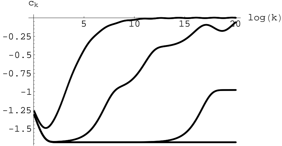
FIGURE 6. Plot of c_k for \alpha = \frac{1}{2}, \beta = 4, 10, 24, 50 from top to bottom (data obtained with n = 10^6 in (4)).
