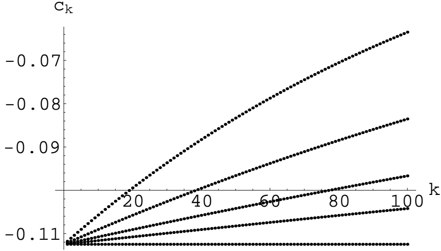
FIGURE 4. Plot of c_k for \alpha = 7/2 and \beta = 4, 5, 6, 7, 20 (from top to bottom).
