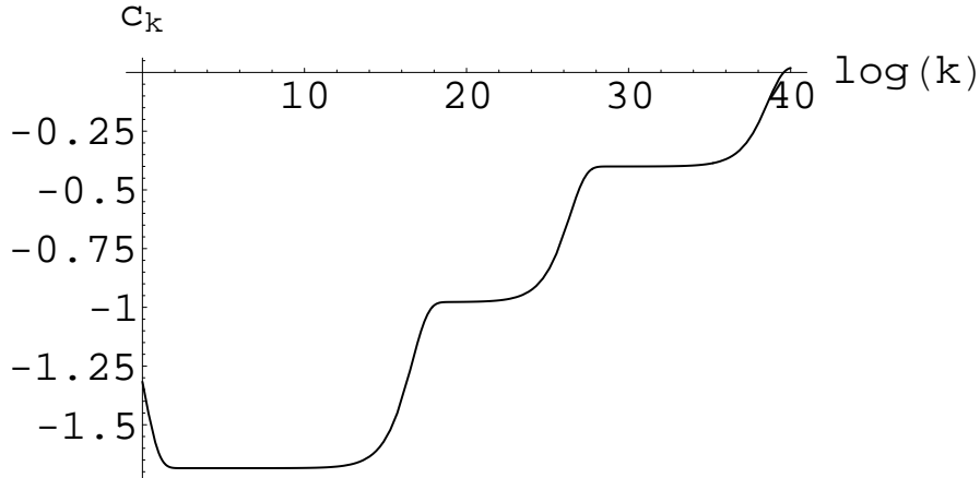
FIGURE 8. Plot of c_k for \alpha = \frac{1}{2}, \beta = 24 (data obtained with n = 10^6 in (4)).
