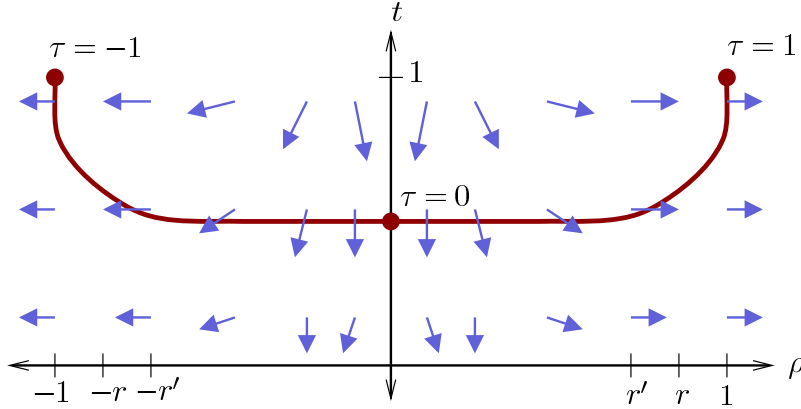
Figure 5. The path (t(\tau), \rho(\tau)) transverse to the vector field of (3.9).
