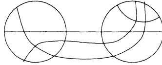
FIGURE 30. An example of a chord diagram considered in Proposition 3.16.
