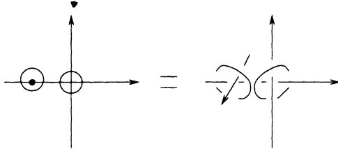
FIGURE 11. Some abbreviation conventions for drawing the next figure.
