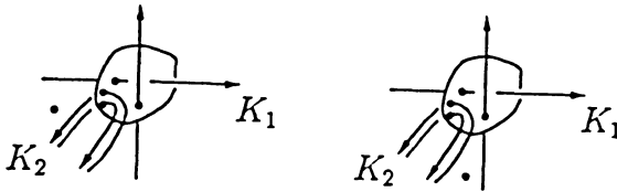
FIGURE 18. Shown here are the links E_1 and E_2 of equation (16).
