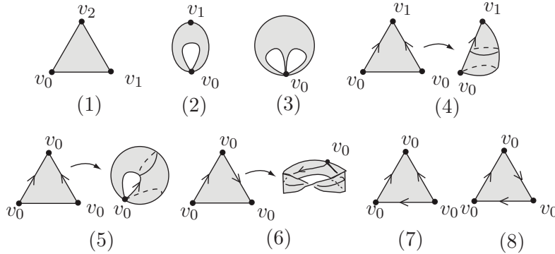
Figure 1: Possible configurations for faces in a triangulation.
