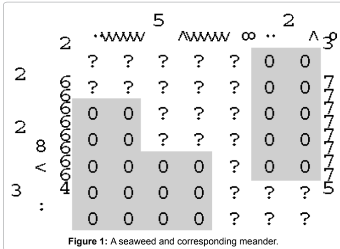
Figure 1: A seaweed and corresponding meander.
