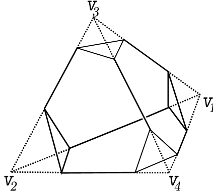
FIGURE 1. Generalised hyperbolic tetrahedron
