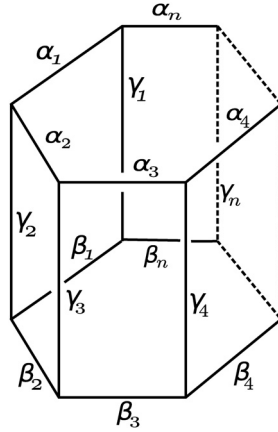
FIGURE 4. The prism \Pi_n(\vec{\alpha}_n, \vec{\beta}_n, \vec{\gamma}_n)
