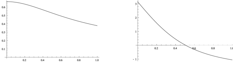
FIGURE 11. Left: Vol T_5 , right: \frac{\partial \Phi}{\partial \ell} , both as functions of \ell
