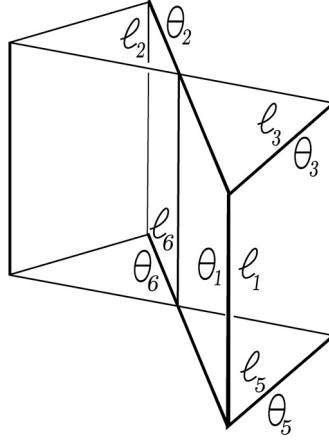
FIGURE 10. Parametrising the “butterfly” prism depicted in Fig. 8
