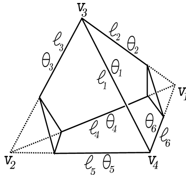
FIGURE 2. Doubly truncated tetrahedron (mild truncation)
