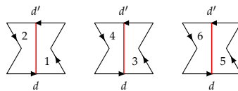
Figure 4: Walls of type d
