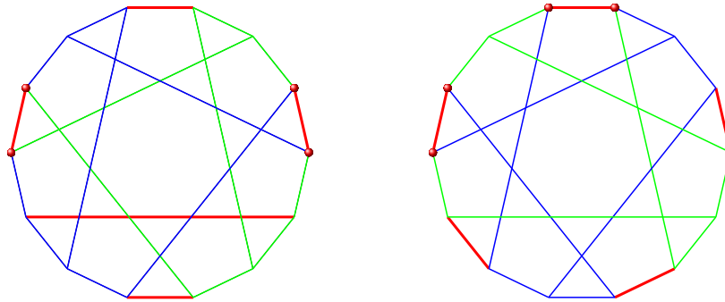
Figure 7: Halving spherical buildings
