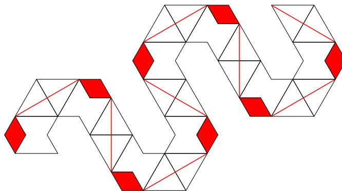
Figure 8: Zigzags in walls
