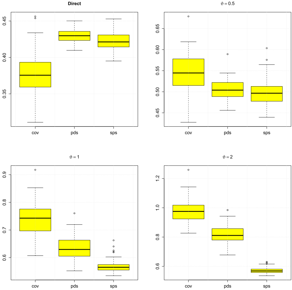
Figure 4. Block diagonal \Sigma : box plots of the estimation errors \|\Sigma_t^o - \Sigma\| for o \in \{\text{cov}, \text{pds}, \text{sps}\} in the case of the convolution model Y = X + \varepsilon with \varepsilon \stackrel{d}{=} \sqrt{W}Z , where Z \sim \mathcal{N}_{20}(0, I_{20}) and W \sim \text{Gamma}(\vartheta) .
