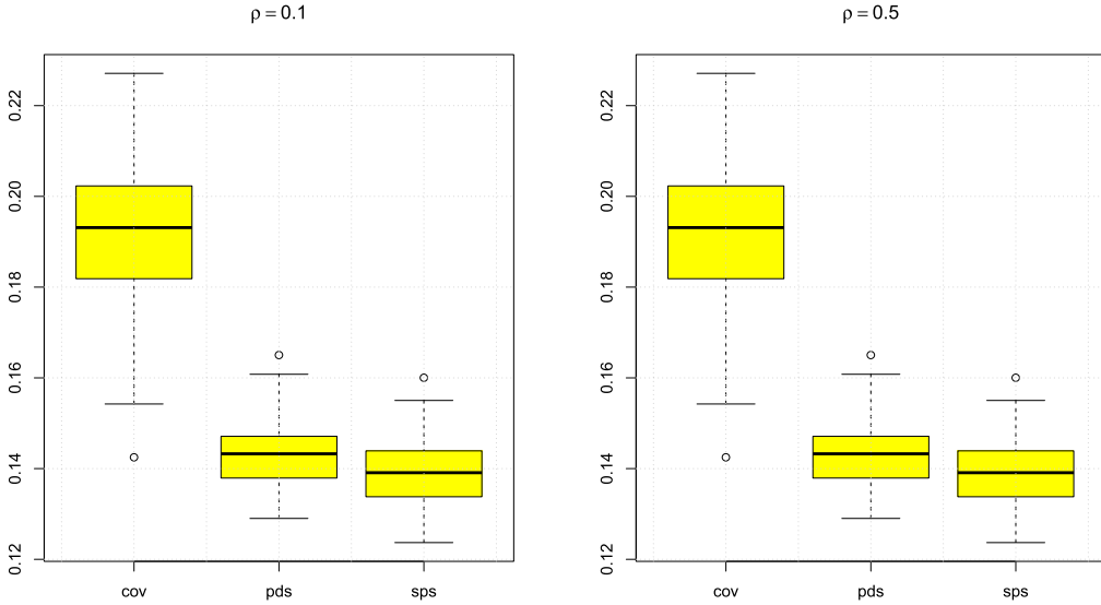
Figure 3. Tridiagonal \Sigma : box plots of the estimation errors \|\Sigma_\tau^o - \Sigma\| for o \in \{\text{cov}, \text{pds}, \text{sps}\} in the case of the convolution model Y = X + \varepsilon with \varepsilon \stackrel{d}{=} Z , where Z \sim \mathcal{N}_{20}(0, \rho I_{20}) .
