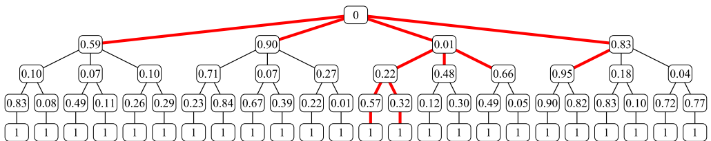
Figure 1. A tree for L = 4 and x = 0 . The bold lines (also red in the online version) indicate the directed paths going down from the root (at the top) and which visit an increasing sequence of numbers. There are \Theta = 2 paths going all the way down to the leaves of the tree.
