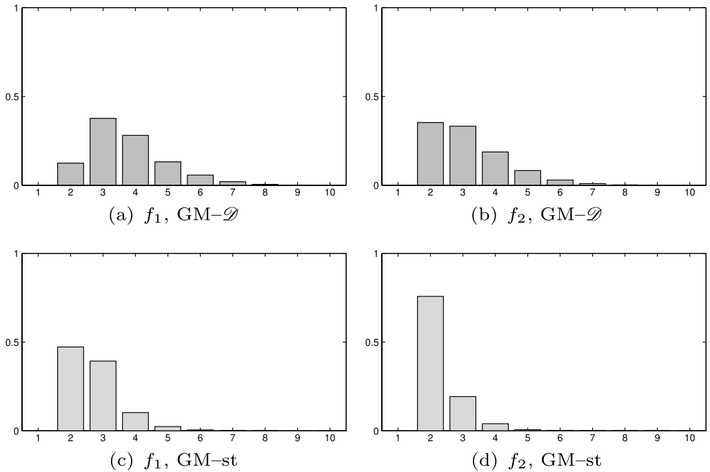
Figure 2. GM- \mathcal{D}(c, z, P_0) (top row) vs. GM-st( \sigma, z, P_0 ) (bottom row) mixture with random c and \sigma , respectively: posterior distributions of the number of clusters K_X and K_Y .
