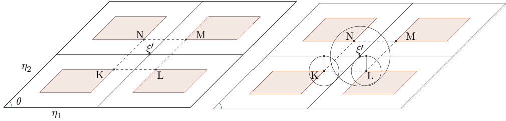
Figure 2. (Left) B_{-r/\beta}(\mathcal{X}) + \mathcal{L} ; (Right) Balls B(\xi', 2r/\beta), B(K, r/\beta) and B(L, r/\beta) .
