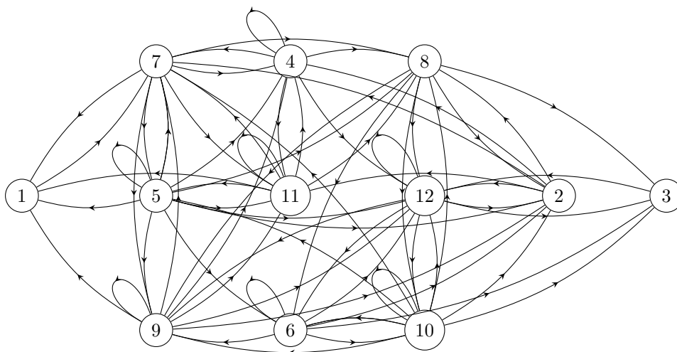
Figure 7. Sofic graph for 3-fold rotation.
