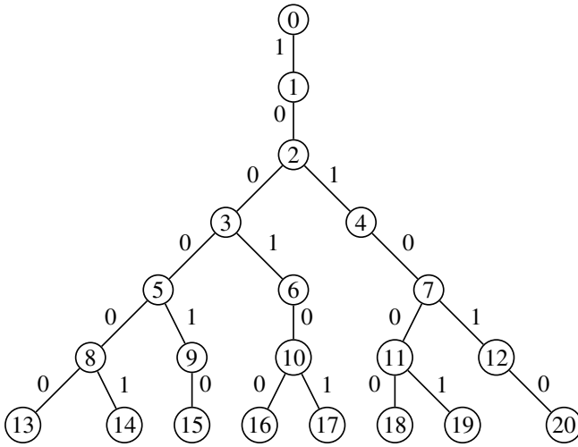
Figure 1. The Zeckendorf tree up to n = 20 .
