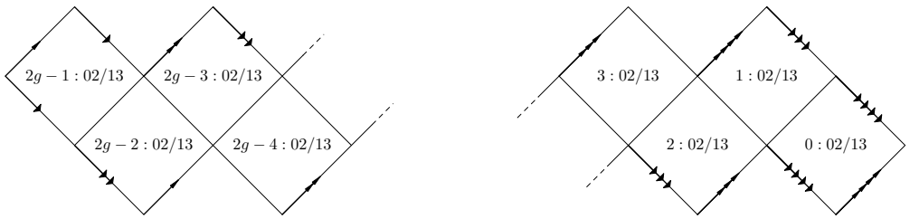
Figure 18: Genus- g splitting surface in \mathcal{B}_g with only 2g quadrilaterals.
