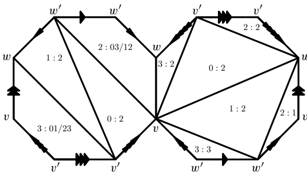
Figure 20: A genus-2 quadrilateral fundamental normal surface with only two quadrilaterals.
