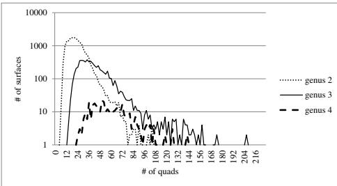
Figure 24: Number of quadrilaterals in the incompressible surfaces (left) and in all Q -extremal surfaces (right) of the Hodgson–Weeks census.
