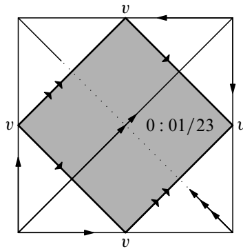
Figure 17: An edge link in the 2–vertex, 1–tetrahedron triangulation of the 3–sphere — a torus consisting of a single quadrilateral.
