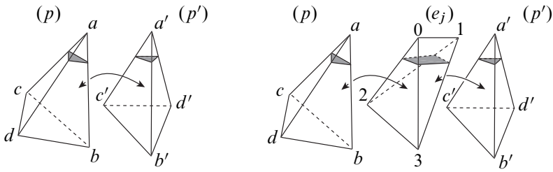
Figure 8: The edge e_j of the frame \lambda lies in the face common to tetrahedra (p) and (p') . An inflation at the face \sigma opens up the identification between (p) and (p') and adds a new tetrahedron (e_j) along with induced face identifications between (p) and (e_j) and (e_j) and (p') . Left: (p)(abc) \leftrightarrow (p')(a'b'c') . Right: (p)(abc) \leftrightarrow (e_j)(032) and (e_j)(132) \leftrightarrow (p')(a'b'c') .
