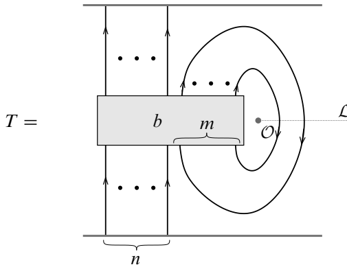
Figure 4: Markov presentation.
