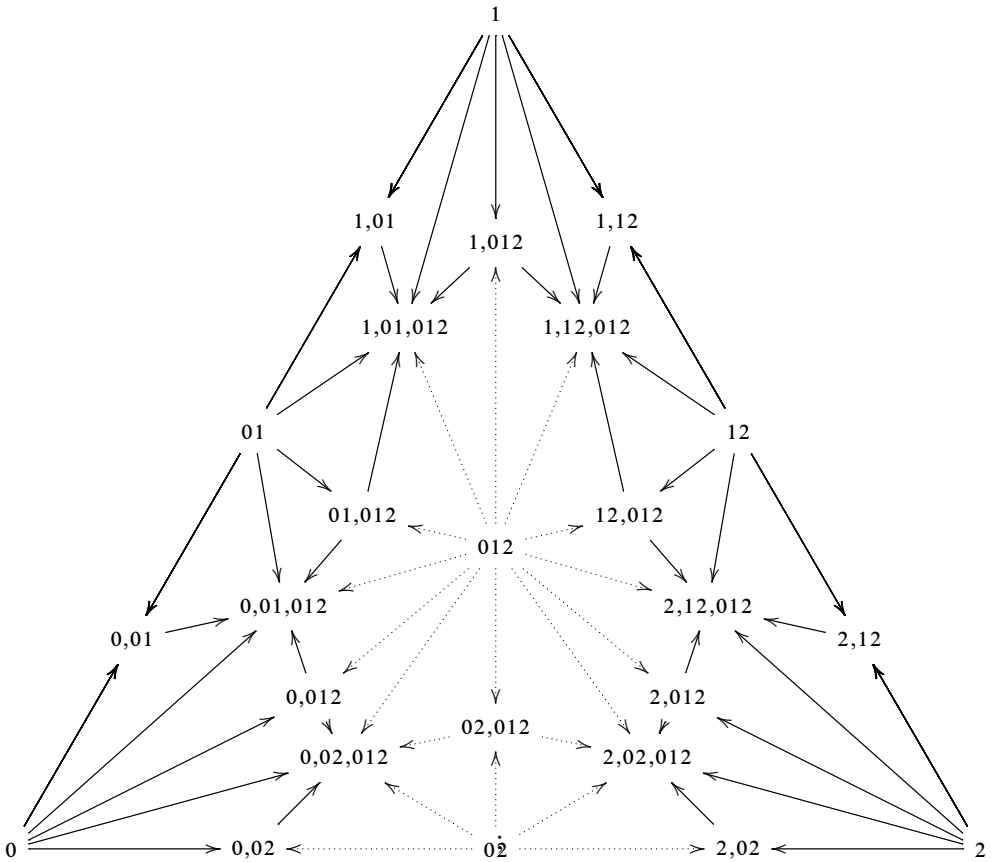
Figure 1: Decomposition of the poset \mathbf{P Sd} \Delta[2] . The dark arrows form the poset \mathbf{P Sd} \Delta^1[2] , while its up-closure Outer consists of all solid arrows. The poset Center consists of all the triangles emanating from 012; these triangles all have two dotted sides emanating from 012. The poset Comp consists of the four triangles at the bottom emanating from 02; these four triangles each have two dotted sides emanating from 02. The geometric realization of all triangles with at least two dotted edges, namely |N(\mathbf{Comp} \cup \mathbf{Center})| , is topologically deformation retracted onto the solid part of its boundary.
