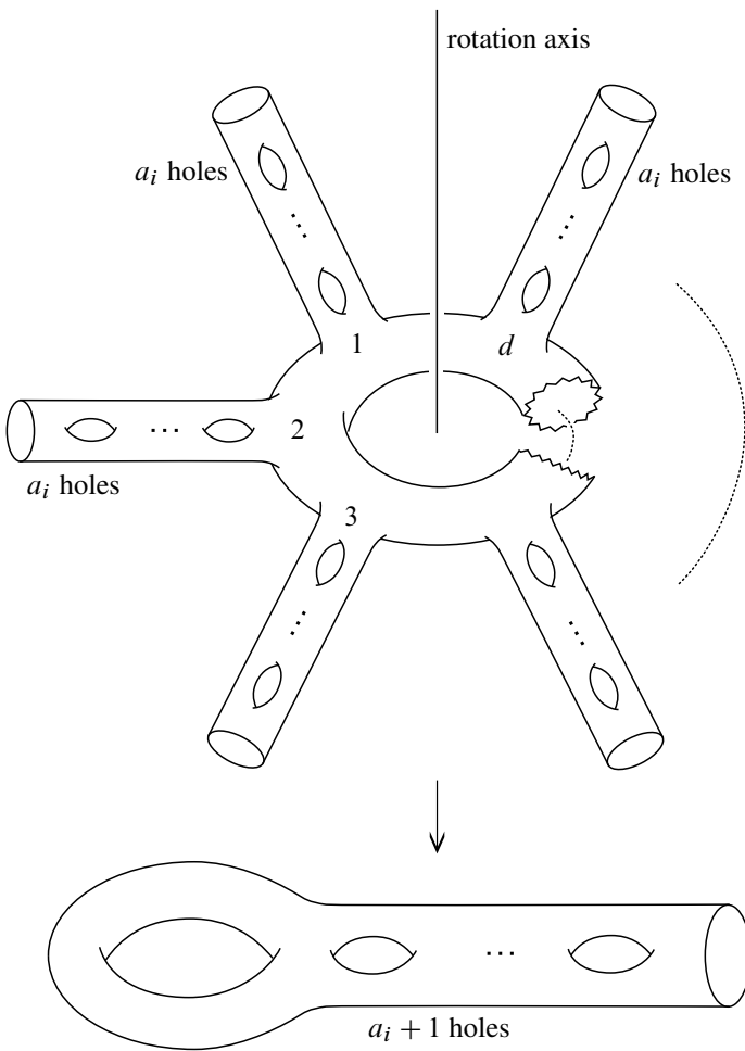
Figure 4: Fixed point free action of \mathbf{Z}/d\mathbf{Z}
