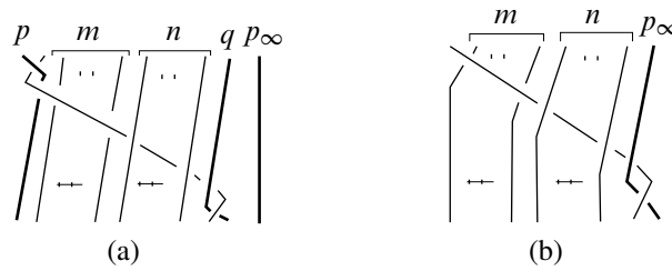
Figure 10: Spherical braids (a) \hat{\beta}_{m,n}^+ and (b) \hat{\sigma}_{m,n}
