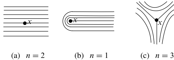
Figure 4: Local picture of a singular foliation
