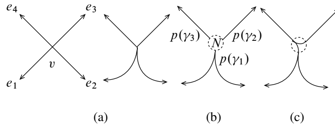
Figure 8: Example of a graph smoothing
