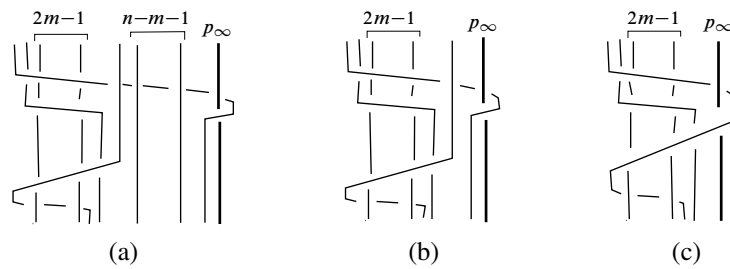
Figure 16: After (m - 1) inductive steps: (a) n \geq m + 2 (b) n = m + 1 (c) n = m
