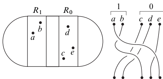
Figure 27: Periodic orbit with the code 10010 and its braid representative
