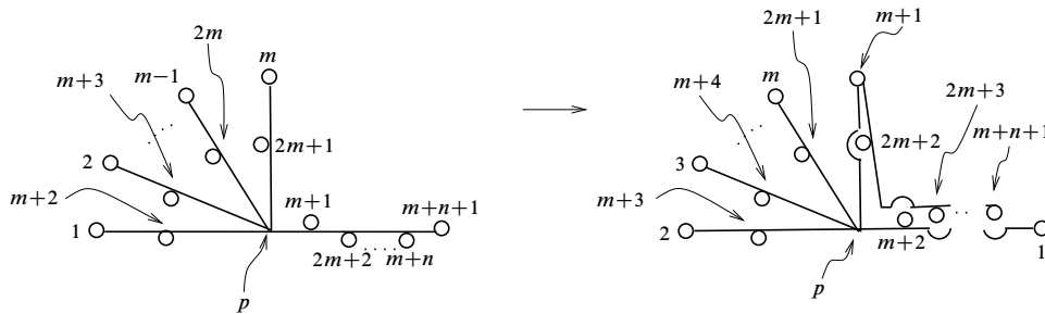
Figure 19: Graph map \mathfrak{h}_{m,n} for \phi_{\sigma_{m,n}}
