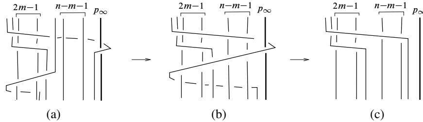
Figure 18: General case
