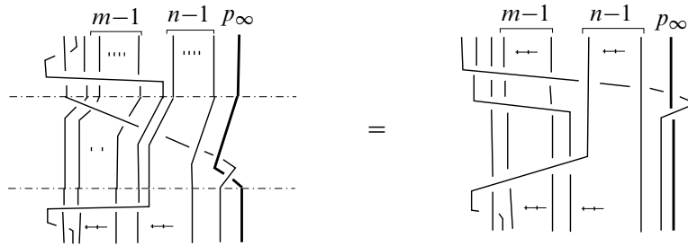
Figure 14: Conjugating \hat{\sigma}_{m,n} : Initial step
