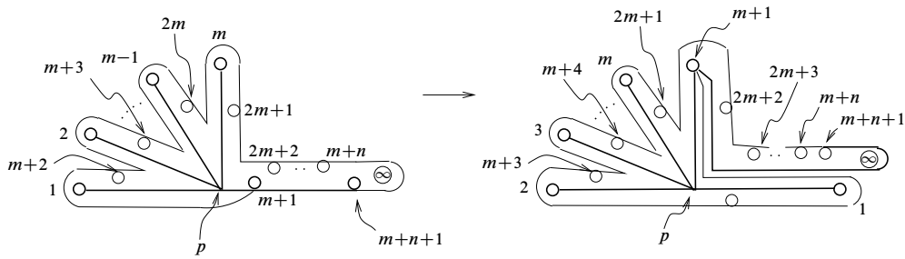
Figure 23: Exchanging the roles of q and p_\infty for g'_{m,n} : \infty in the figure indicates p_\infty
