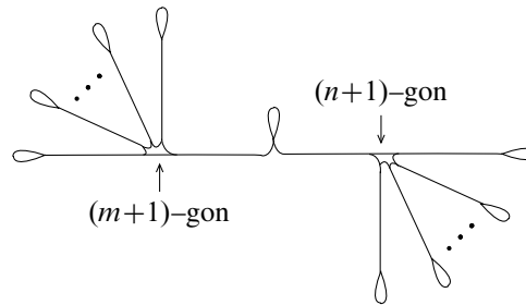
Figure 20: Train track \tau_{g_{m,n}}
