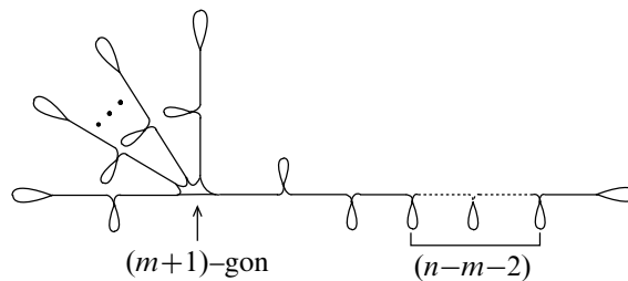
Figure 21: Train track \tau_{h_{m,n}}
