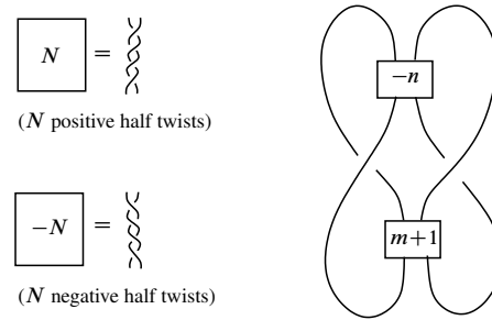
Figure 28: Two-bridge link associated to \beta_{m,n}
