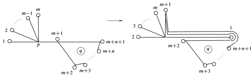
Figure 22: Graph map \mathfrak{g}'_{m,n} for \phi_{m,n}
