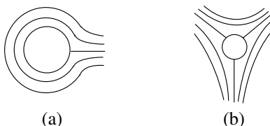
Figure 5: Leaves of a singular foliation near a boundary component
