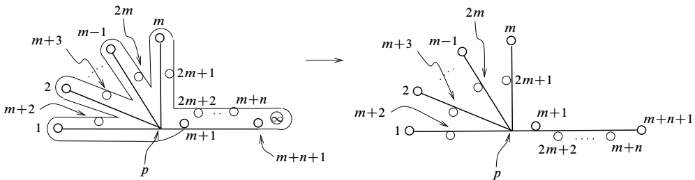
Figure 24: Identifying edges of G'_{m,n} with edges of H_{m,n}
