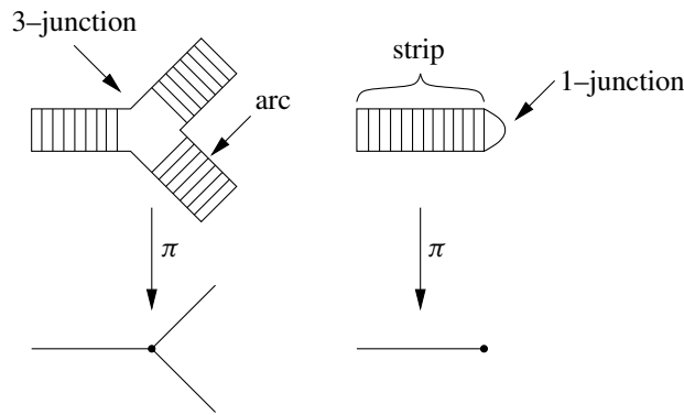
Figure 7: Fibred surface
