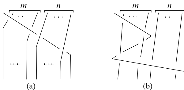
Figure 1: Braids (a) \beta_{m,n} and (b) \sigma_{m,n}
