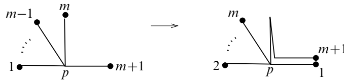
Figure 25: Graph map \tau_m: \Gamma_m \rightarrow \Gamma_m
