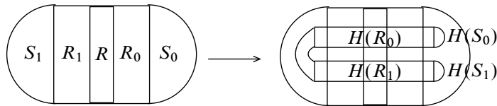
Figure 26: Smale-horseshoe map
