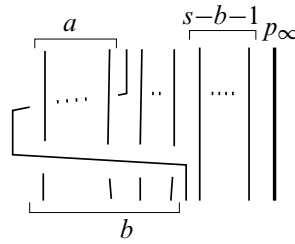
Figure 13: Spherical braid \tau_{a,b} \in \mathcal{B}(S^2; \mathcal{S}, \{p_\infty\})
