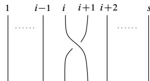
Figure 2: Braid generator \sigma_i
