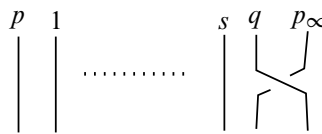
Figure 11: Spherical braid \nu : Switching the roles of p_\infty and q
