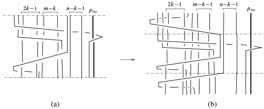
Figure 15: Induction step
