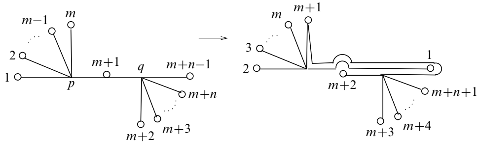
Figure 12: Graph map g_{m,n} for \phi_{\beta_{m,n}}
