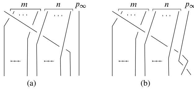
Figure 3: Images of (a) \beta_{m,n} and (b) \sigma_{m,n} in \mathcal{B}(S^2; \mathcal{S}, \{p_\infty\})
