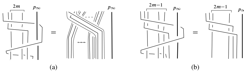
Figure 17: (a) reducible and (b) periodic cases
