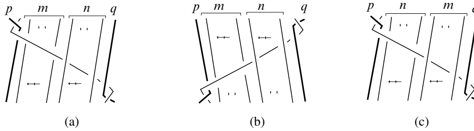
Figure 9: Symmetry of \beta_{m,n}^+
