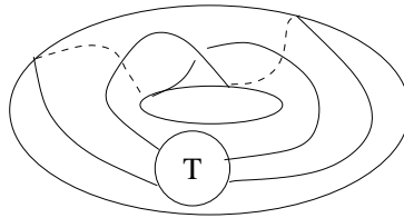
Figure 5: Representation: (F, K_v)
