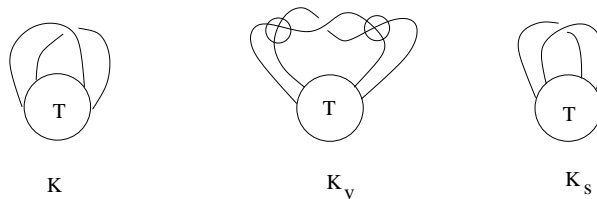
Figure 3: K , K_s and the virtualized diagram: K_v
