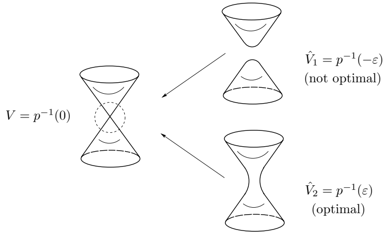
Figure 1: p(x, y, z) = x^2 + y^2 - z^2
