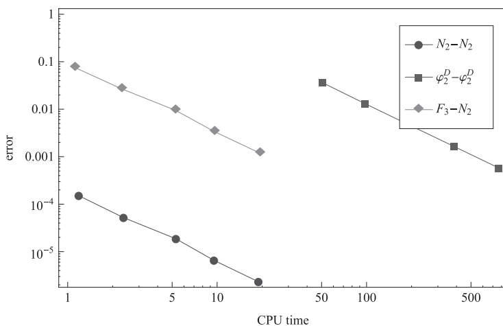
Figure 6: case 3; u(x) = N_3(3x)
