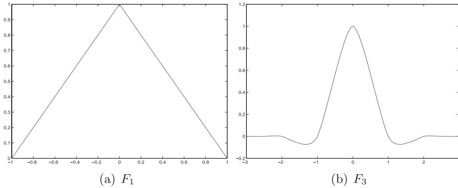
Figure 1: Deslauriers–Dubuc fundamental functions
