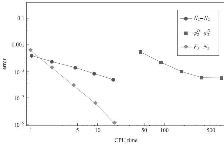
Figure 4: case 1; u(x) = x^5(1 - x)^5
