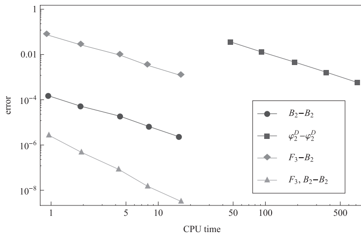
Figure 9: case 3; u(x) = N_3(3x)
