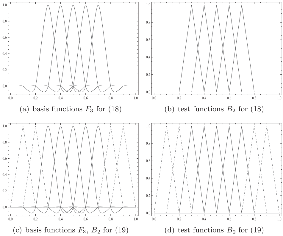
Figure 8: basis and test functions for (18) and (19)
