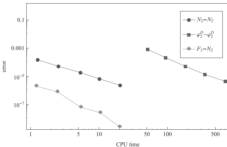
Figure 7: case 4; u(x) = N_3(10x/3 - 1/6) (supp u = [1/20, 19/20] )
