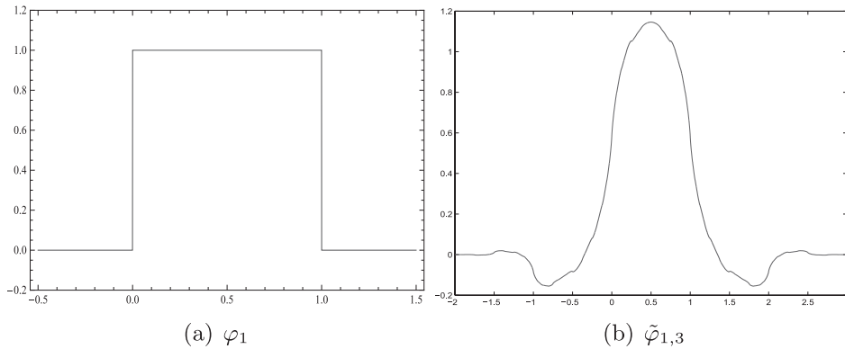
Figure 3: Biorthogonal B-spline functions
