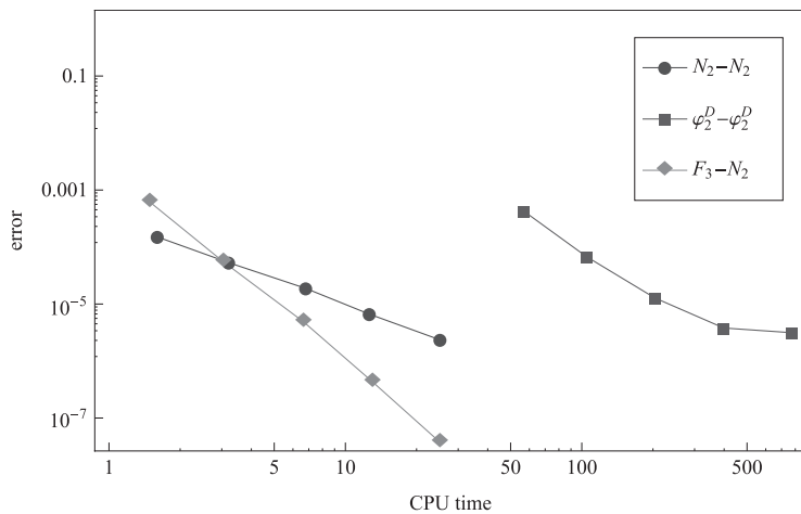
Figure 5: case 2; u(x) = N_5(5x)
