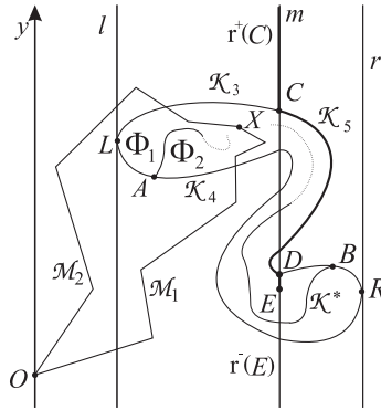
Figure 5. There is no point from the set \text{Ex}(\Phi_1) \cap \text{Ex}(\Phi_2) \cap \text{In}(\Phi) .
