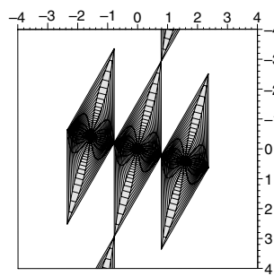
(f) Projection of (e) onto xy -plane
