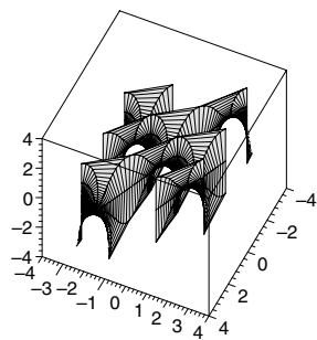
(c) Five pieces of Scherk's Slanted Surface ( m = e^{i\pi/4} )
