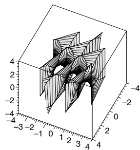
(e) Five pieces of Scherk's Slanted Surface ( m = e^{i\pi/6} )
