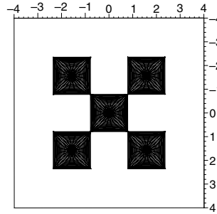
(b) Projection of (a) onto xy -plane
