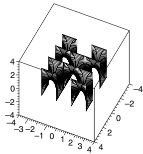
(a) Five pieces of Scherk's First Surface ( m = e^{i\pi/2} )
