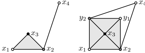
FIGURE 1. The simplicial complexes \Delta (left) and \Delta_\chi (right).
