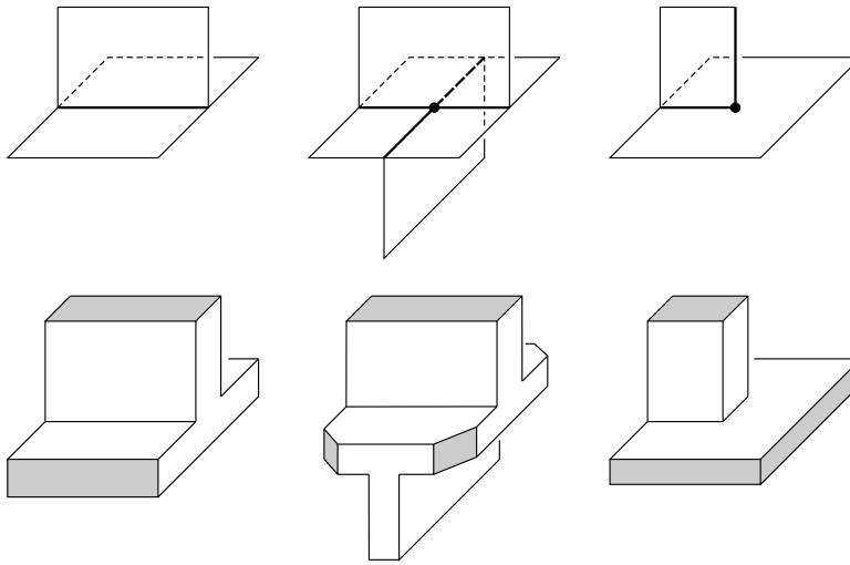
Figure 8. Blocks obtained by thickening fragments of a neighborhood of the union of the triple lines.
