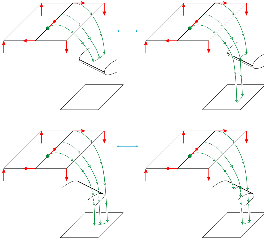
Figure 16. Catastrophes corresponding to a transition orbit being also once concavely tangent to the boundary, with an obvious transversality condition. These pictures refer to an incoming transition orbit, but the analogue catastrophes involving outgoing transition orbits must also be taken into account.
