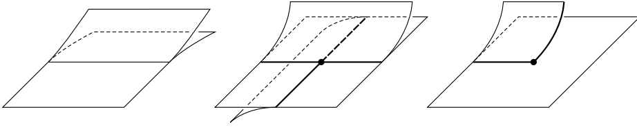
Figure 7. A polyhedron locally as in Figure 5 sitting in a branched fashion in a 3-manifold. Any mirror image in 3-space of these figures is also allowed.
