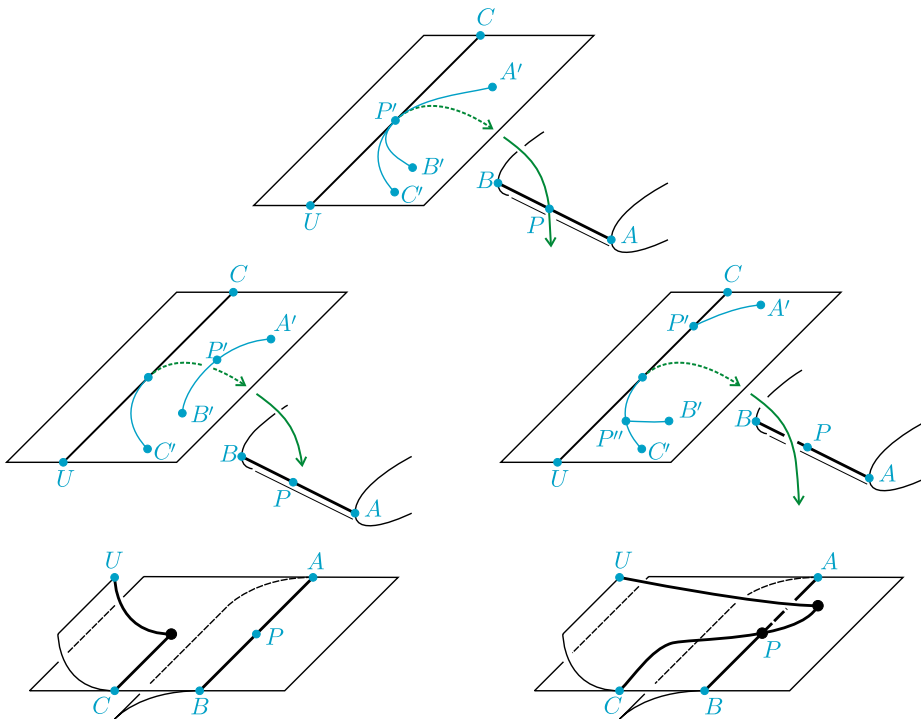
Figure 22. From a catastrophe involving concave tangency of an incoming transition orbit to a spike-sliding in the associated in-backward stream spine.
