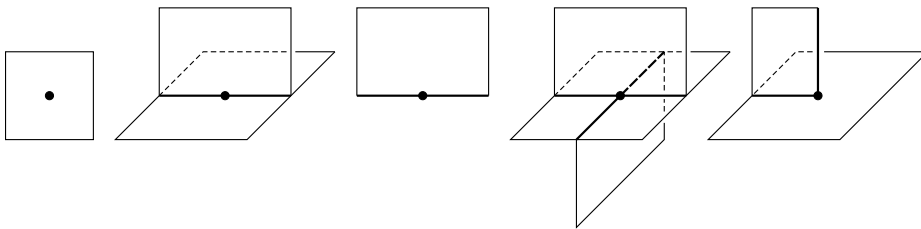
Figure 5. Local aspect of a stream spine.
