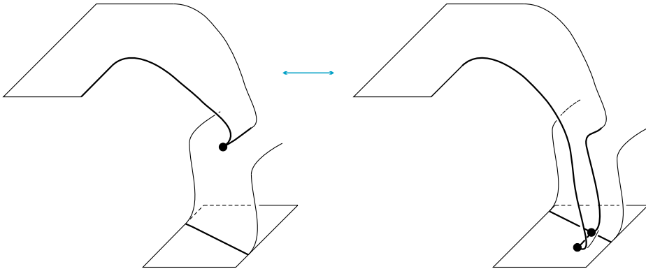
Figure 21. From a catastrophe involving concave tangency of an incoming transition orbit to a spike-sliding in the associated out-forward stream spine.
