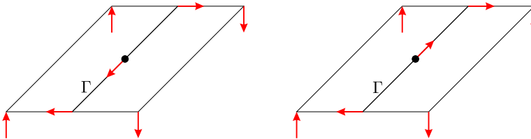
Figure 2. Types of transition points: on the left v points from the concave to the convex portion of \Gamma ; on the right v points from the convex to the concave portion of \Gamma ; note that mirror images in 3-space of these configurations should also be taken into account (namely, the figures are unoriented).
