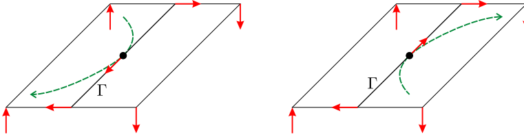
Figure 3. Orbits through the transition points for the field obtained by projecting v to a vector field tangent to \partial M .
