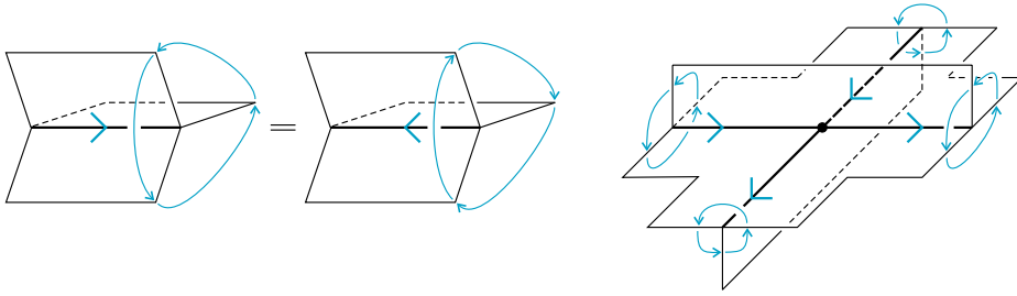
Figure 6. Screw orientation along a triple line and compatibility at vertices.
