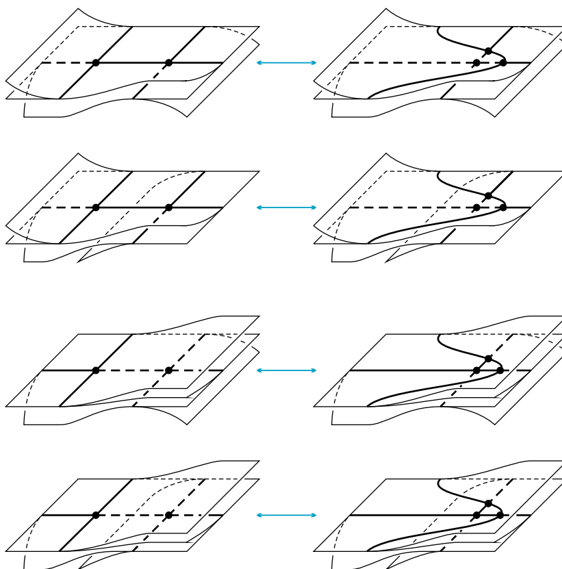
Figure 19. The 2 \leftrightarrow 3 sliding moves.
