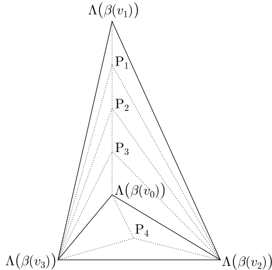
Figure 1: Polytope of \mathbb{P}(1, 3, 4, 4) and of the crepant resolution Z
