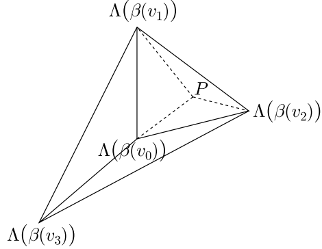
Figure 2: Polytope of \mathbb{P}(1, 1, 1, 3) and a crepant resolution
