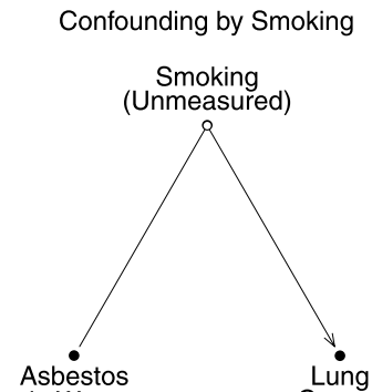
FIG. 2. Smoking as an unmeasured confounder: the noncausal association between asbestos in the water and lung cancer is explained by the associations with smoking.
