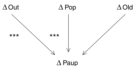
FIG. 1. Yule’s model; metropolitan unions, 1871–1881.
