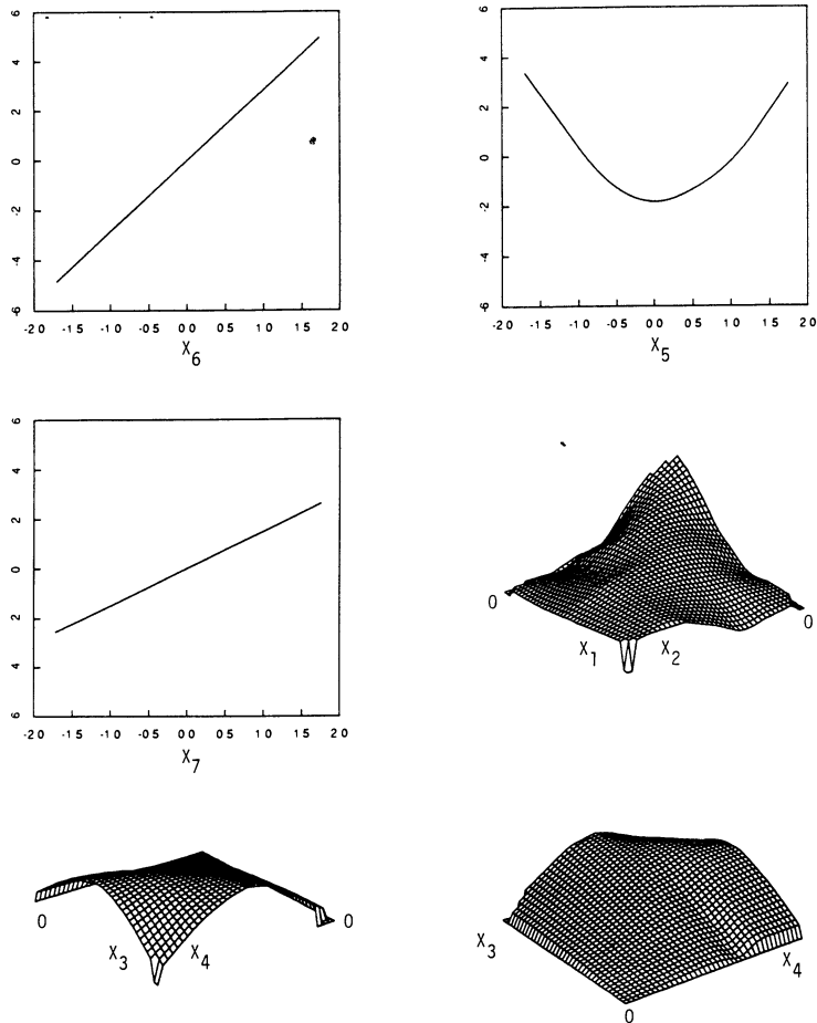
FIG. 13. ANOVA functions for the ten-variable version of the second example in Section 4.6.
