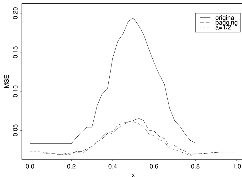
FIG. 8. Mean squared error of stumps \hat{\theta}_n(x) in (3.1) (solid line) and its (su-)bagged version \hat{\theta}_{n;SB(m)}(x) for x \in [0, 1] . Sample size n = 100 and subsampling size m = \lfloor an \rfloor . Everything multiplied by the factor 1/(\beta_u^0 - \beta_\ell^0)^2 = 1/2.25 to obtain (asymptotically) the scale from Figure 7.
