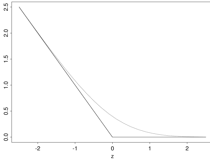
FIG. 5. MARS basis function from (2.10) at x = x_n(0) = d^0 as in (2.14). Function g(z) (solid line) and g_B(z) (dotted line) from Proposition 2.4, defining the asymptotics of \hat{\theta}_n(x_n(0)) and its bagged version, respectively.
