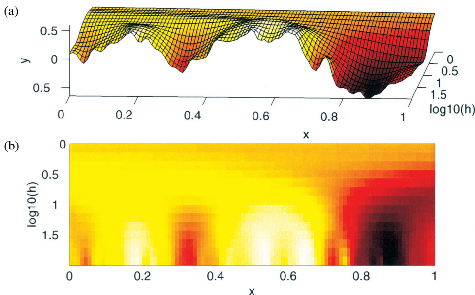
FIG. 3. Figure 3a shows a family of Nadaraya-Watson smooths, similar to Figure 1b, for the data of Figure 1a, but now panels are shaded using a “temperature” color scale. Projection of these colors into the plane is shown in Figure 3b, which shows how (one dimensional) heat diffuses in time.
