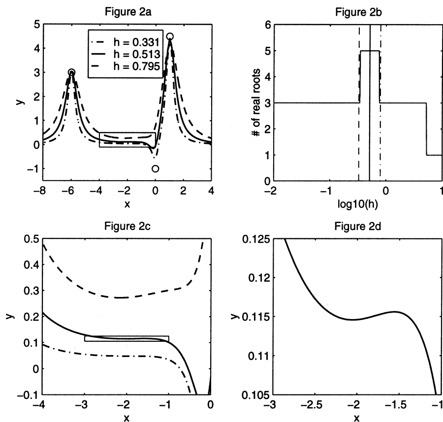
FIG. 2. Counterexample showing that the Cauchy kernel does not satisfy the causality property. A three point regression data set is shown as circles in Figure 2a, together with 3 Cauchy kernel smooths. Figure 2b shows the numbers of real roots of the derivative, as a function of the bandwidth, with the 3 smooths in Figure 2a represented as vertical bars with the same line types. Figure 2c and 2d are successive enlargements of the regions shown as boxes in Figures 2a and 2c respectively.
