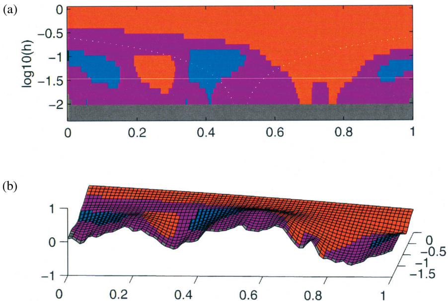
FIG. 5. Figure 5a shows the SiZer map corresponding to the data and the family of smooths shown in Figure 1b. This shows which modes in the smooths are significant, and which are spurious sampling artifacts. Figure 5b shows the family surface with panels shaded according to the SiZer colors.
