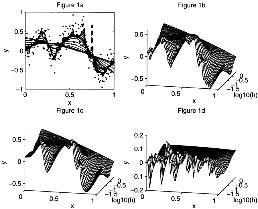
FIG. 1. Simulated regression example showing scale space ideas. Figure 1a shows the target curve as the dashed line, the data as small dots, and a family of local linear smooths as thin solid lines, with the Ruppert-Sheather-Wand bandwidth highlighted as the heavy solid line. Figure 1b is the theoretical scale space surface. Figure 1c is the empirical scale space surface, that is, smooths of the target curve. Figure 1d is the “noise surface,” that is, the difference between the surfaces shown in Figures 1b and 1c.
