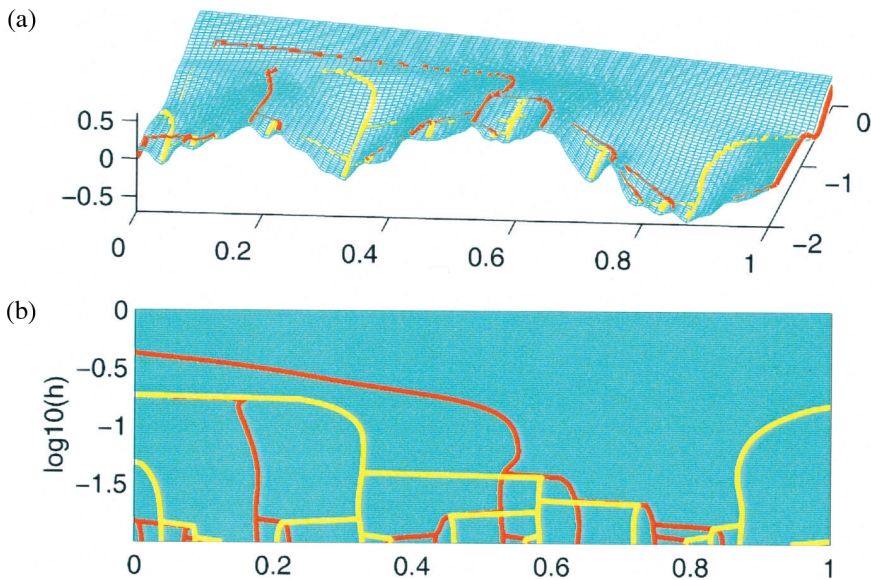
FIG. 4. Figure 4a shows the same family of smooths as in Figure 1b, with modes highlighted in red, and antimodes highlighted in yellow. Figure 4b shows the projection of the red mode locations and the yellow antimode locations into the plane, yielding the mode and antimode trees.
