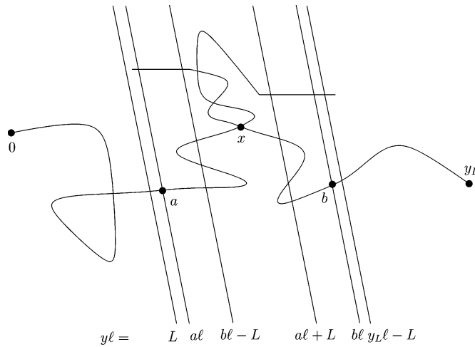
FIG. 1. Sketch for Lemma 6 and the proof of Theorem 1. The paths of two walkers starting in 0 and y_L , respectively, meet in the middle slab \{y : a\ell \leq y\ell \leq b\ell\} in some vertex x before leaving this slab on the side which is opposite to the side of their respective entrance.
