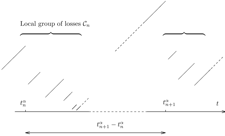
FIG. 1. Evolution of the congestion window size between two groups of losses.
