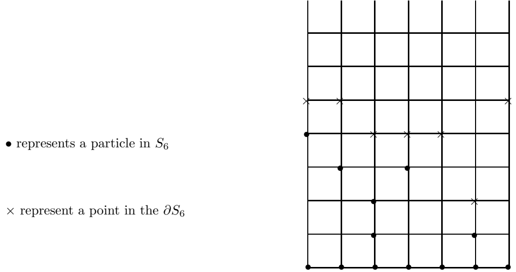
Figure 1: The cluster S_6 and its boundary.
