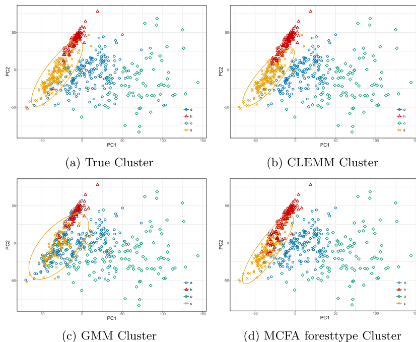
FIG 3. Forest type data. Cluster Visualization, where an observation with very large PC1 score ( x -axis) is removed for better visualization.
