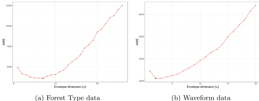
FIG 2. AWE scores for dimension selection in CLEMM.
