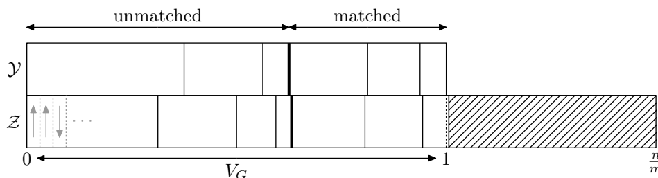
Figure 17: \mathcal{Z}^t consists of blocks representing the cycles C_t , placed in the interval [0, \frac{n}{m}) . Cycles belonging to V_G are placed first, roughly in the interval [0, 1) , and are sorted into those matched with a block of \mathcal{Y}^t and those not. Matched blocks can differ slightly in size. Also \mathcal{Z}^t will after a few steps have an ‘overhang’ since the giant component grows. The hatched part consists of blocks representing cycles with vertices that are not in V_G .
