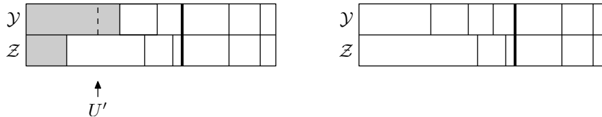
Figure 16: Example when one block is split and one is merged.
