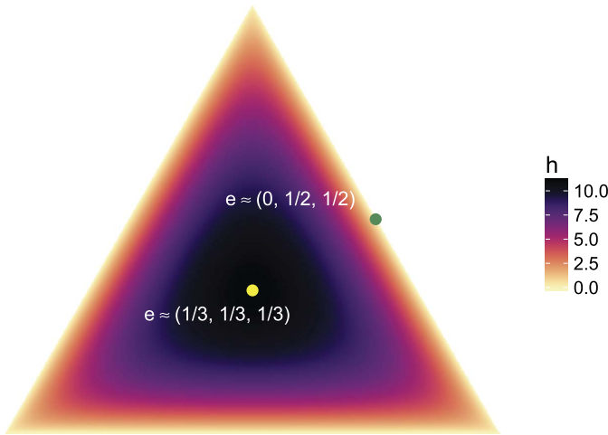
FIG. 1. Ternary plot of optimal h (up to a proportionality constant) as a function of the generalized propensity score vector with J = 3 treatments. Each point in the triangular plane represents a unit with certain values of the generalized propensity scores. The value of each generalized propensity score is proportional to the orthogonal distance from that point to each edge. It is evident that the new weighting scheme emphasizes the centroid region with good overlap, for example, units with e(\mathbf{X}) \approx (1/3, 1/3, 1/3) , and smoothly down-weights the edges, for example, units with e(\mathbf{X}) \approx (0, 1/2, 1/2) .
