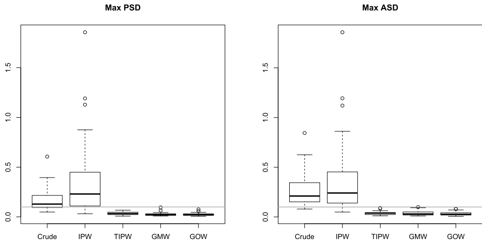
FIG. 2. Boxplots for the maximum population standardized difference (PSD) and maximum absolute standardized difference (ASD) for all health status covariates corresponding to each adjustment method. The gray horizontal line indicates adequate balance at 0.1. Crude: unweighted; IPW: inverse probability weighting; TIPW: inverse probability weighting combined with optimal trimming; GMW: generalized matching weighting; GOW: generalized overlap weighting.
