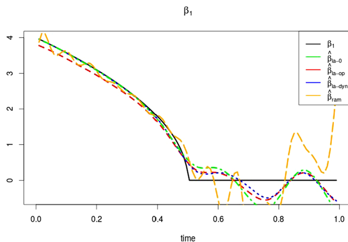
FIG 4. An example of the estimation of \beta_1 (black solid line) with a sample size n = 100 . In green, the estimator without penalization ( \lambda = 0 ); in red, the FREE with optimized parameter \lambda > 0 optimal; in blue, the FREE with the functional optimized parameter \Lambda , and Ramsay's estimator in orange.
